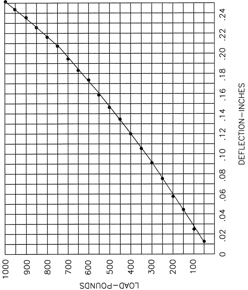
DEFLECTION GRAPH FOR 400N
